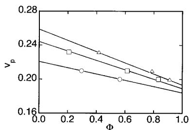
Figure 3. Plots of polymer volume fraction, v_p , versus relative volume of the isotropic phase, \Phi , determined for a mixture of PBLG ( M_w = 6.2 \times 10^4 ) dissolved in DCA/DCE (80/20, w/w): 25 °C (○), 10 °C (□), and 0 °C (△).
