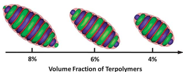
Fig. 9 Multicore micelle structures as a function of the volume fraction of terpolymers for linear ABC terpolymers in a selective solvent with f_A = f_C = 0.40 and \chi_{BS}N = 2.0 . The colors appear as in Fig. 2.
